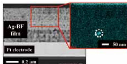
Fig.1 Cross-sectional ADF-STEM image and Ag L \alpha EDX signal mapping of Ag-BF thin film.
